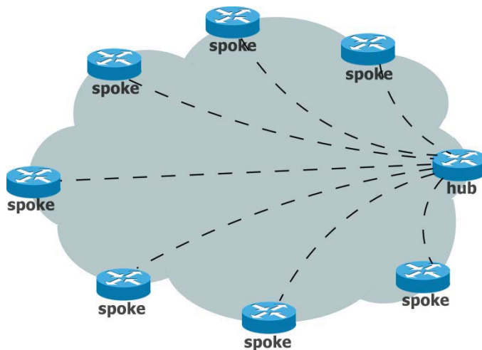
Obr. 2: Hub-and-Spoke topológia
