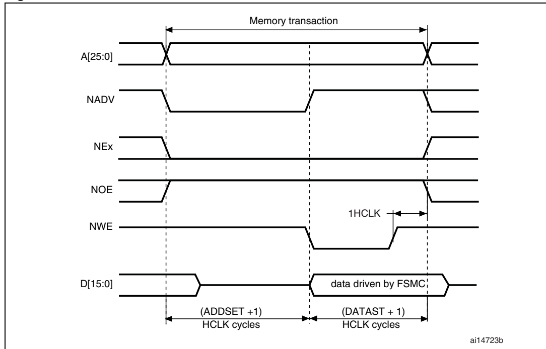
Figure 167. ModeC write accesses
