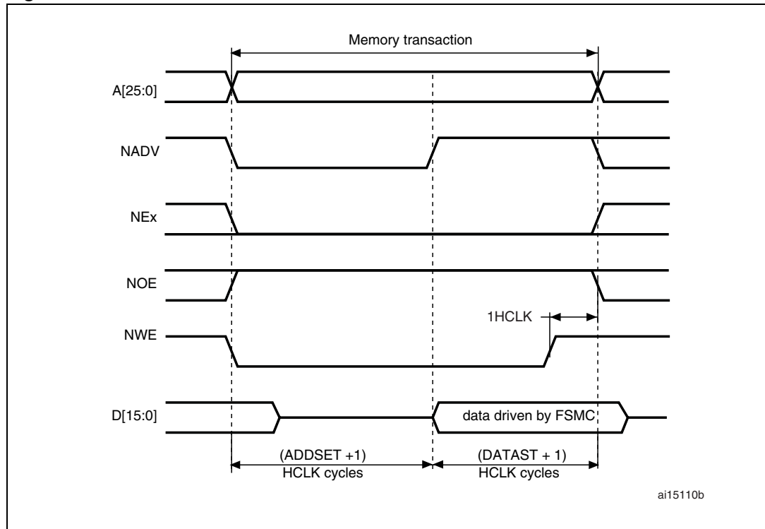
Figure 165. ModeB write accesses
