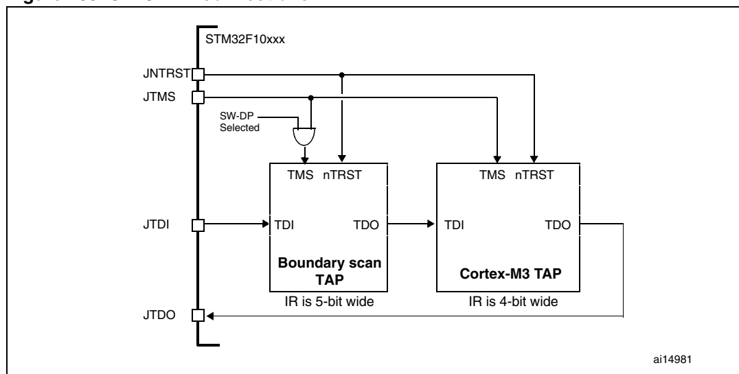
Figure 260. JTAG TAP connections
