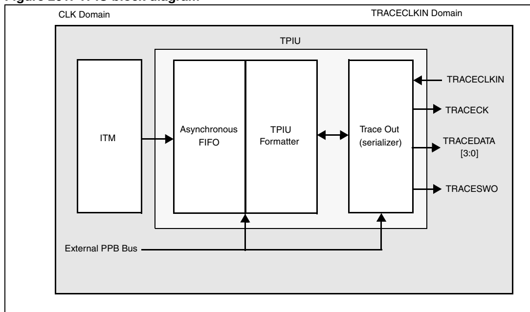
Figure 261. TPIU block diagram
