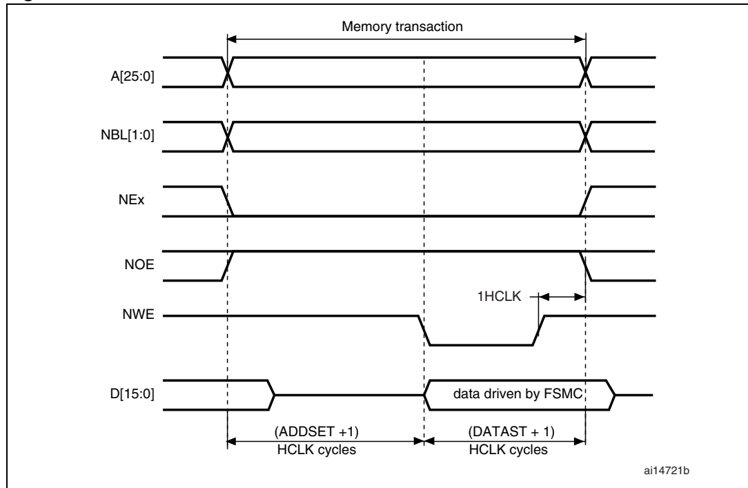
Figure 162. ModeA write accesses
