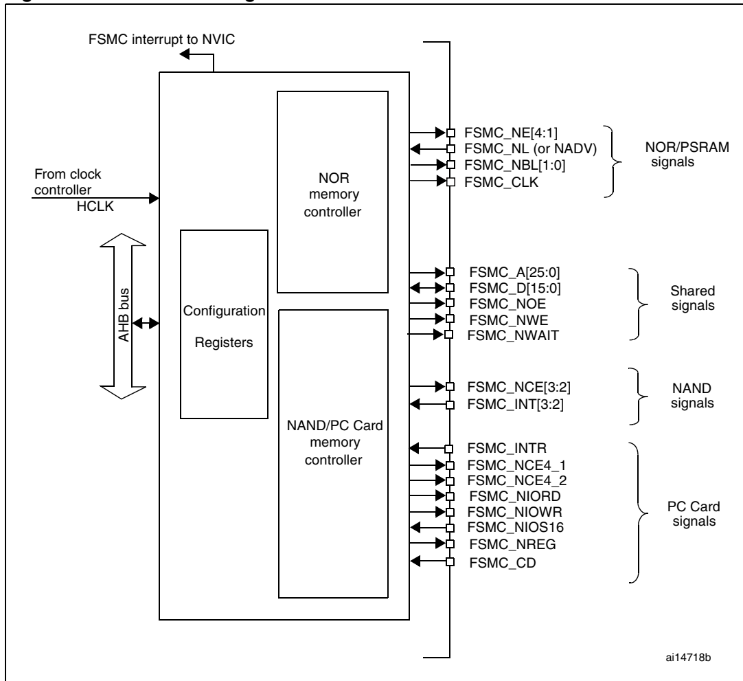
Figure 157. FSMC block diagram
