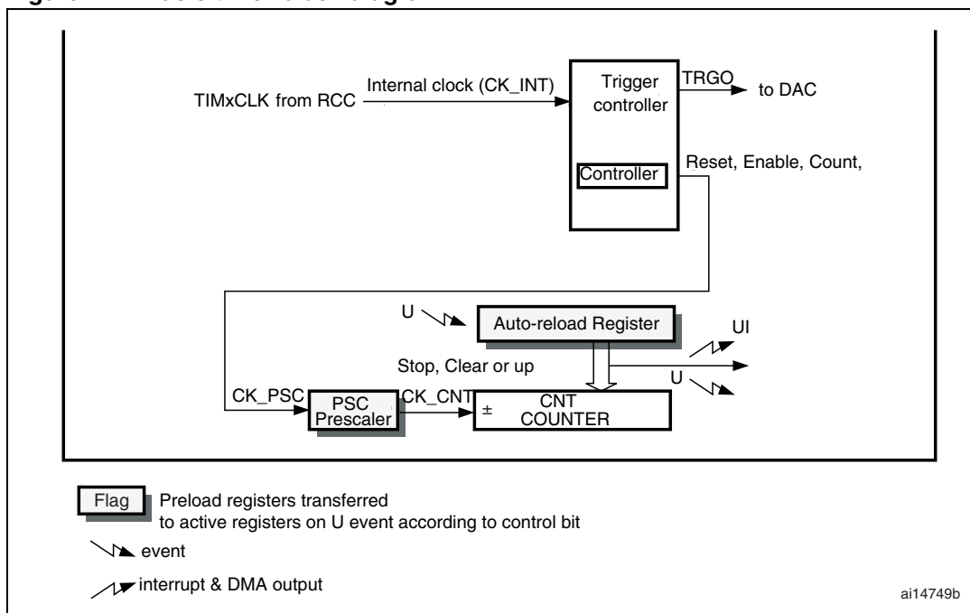
Figure 141. Basic timer block diagram
