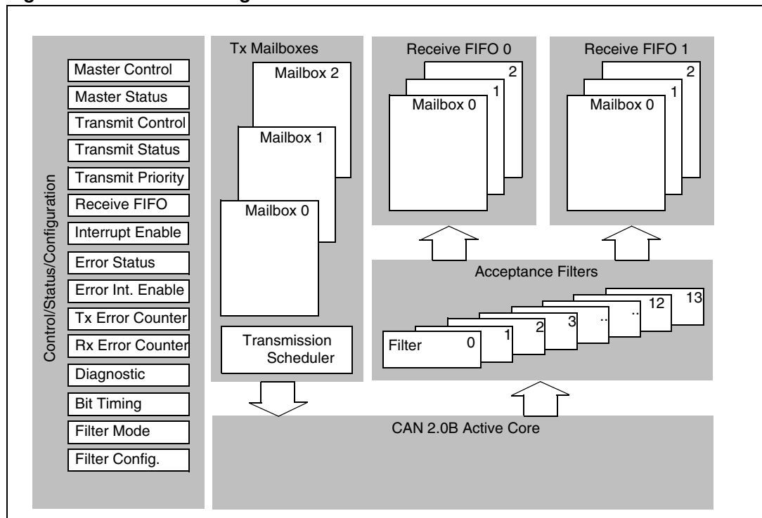
Figure 192. CAN block diagram
