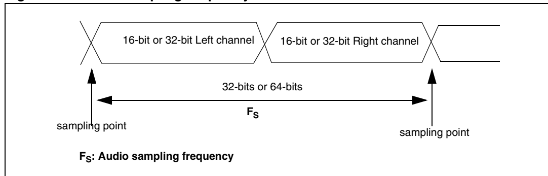
Figure 228. Audio sampling frequency definition
