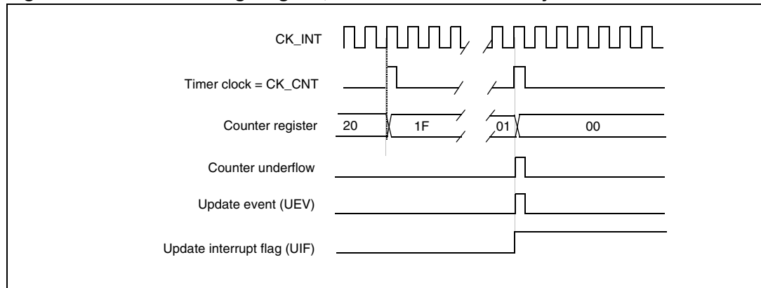
Figure 113. Counter timing diagram, Update event with ARPE=1 (counter underflow)
