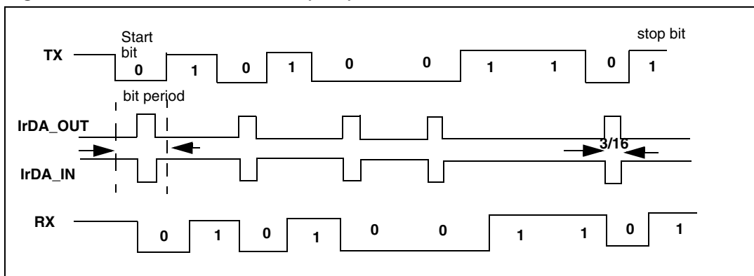
Figure 253. IrDA data modulation (3/16) -Normal Mode
