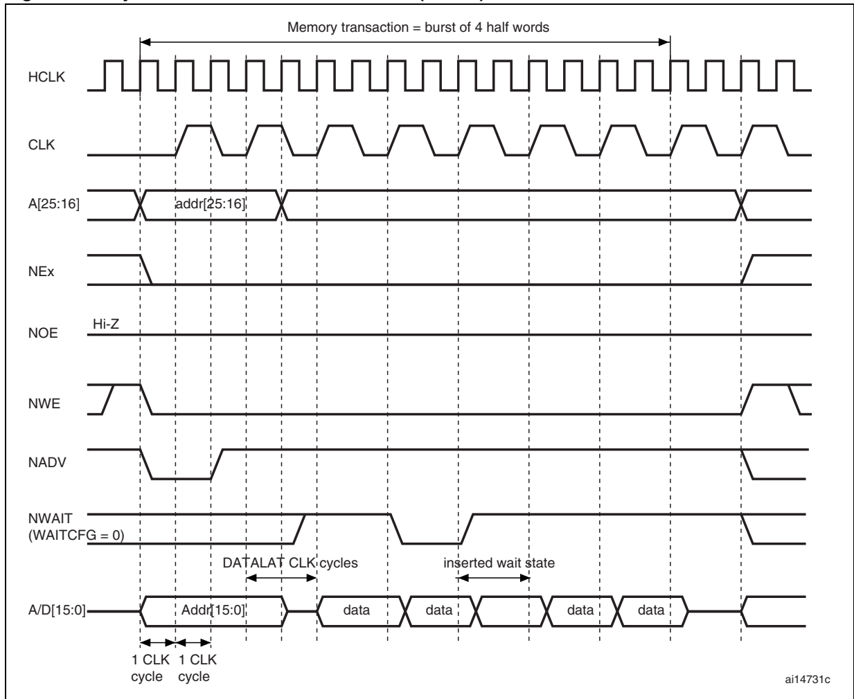
Figure 173. Synchronous write mode - PSRAM (CRAM)
