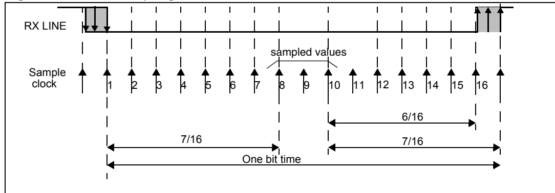
Figure 241. Data sampling for noise detection
