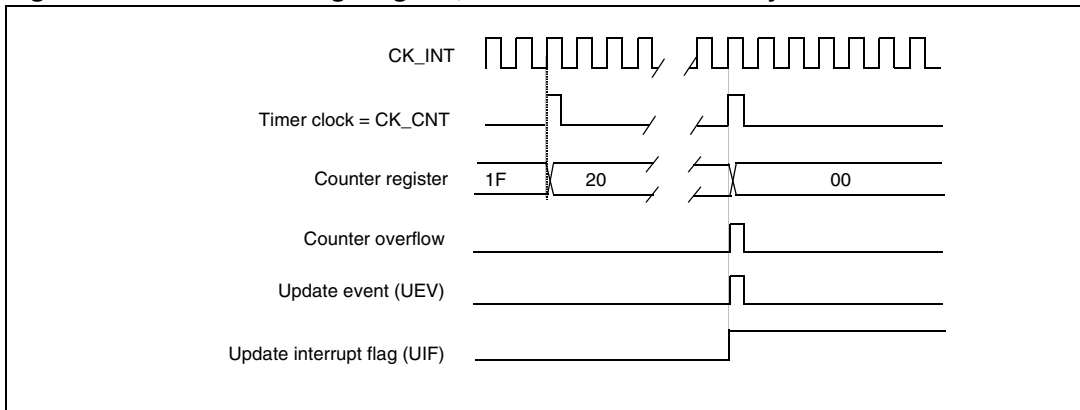
Figure 102. Counter timing diagram, Update event when ARPE=0 (TIMx_ARR not preloaded)
