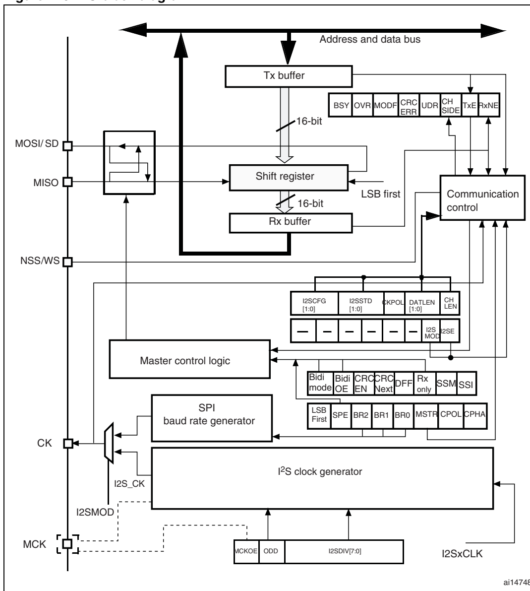
Figure 210. I 2 S block diagram
