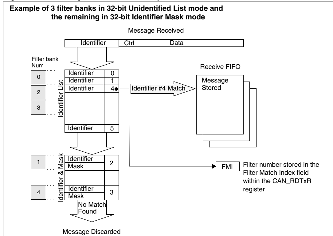
Figure 201. Filtering mechanism - example
