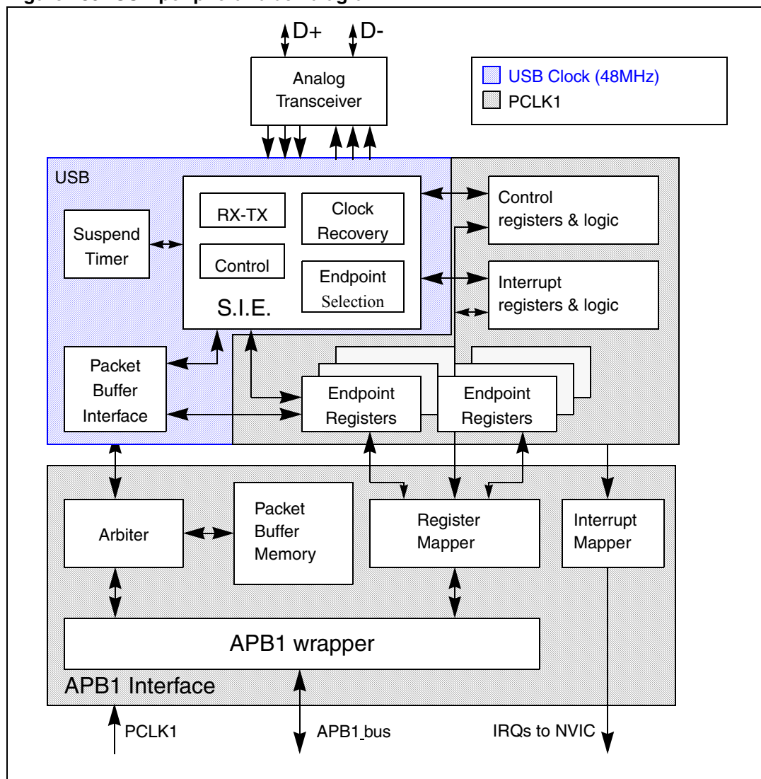
Figure 189. USB peripheral block diagram
