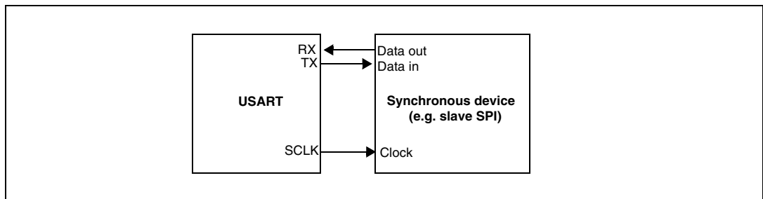
Figure 246. USART example of synchronous transmission
