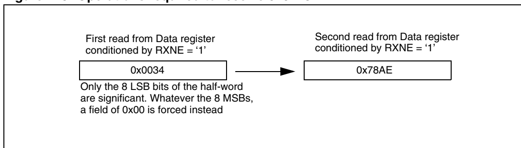
Figure 223. Operations required to receive 0x3478AE
