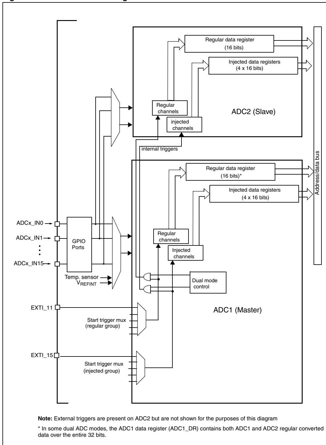
Figure 28. Dual ADC block diagram
