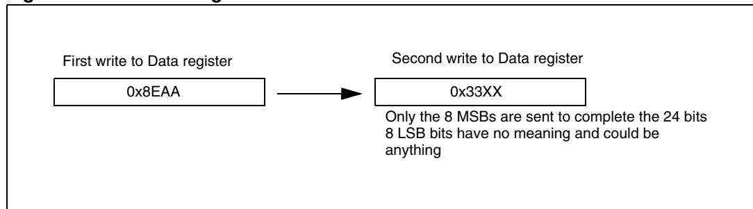
Figure 213. Transmitting 0x8EAA33
