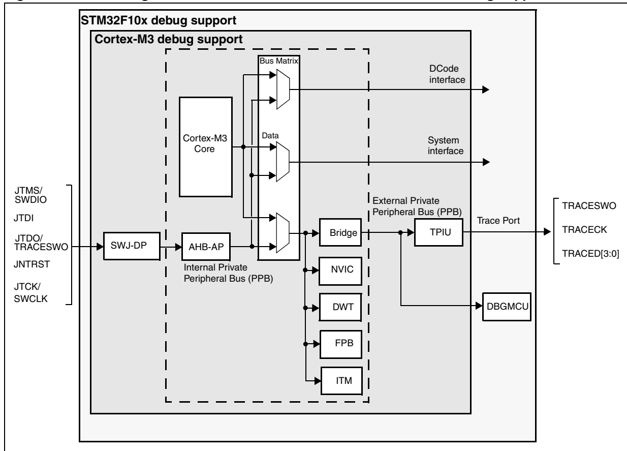
Figure 258. Block diagram of STM32F10xxx-level and Cortex-M3-level debug support
