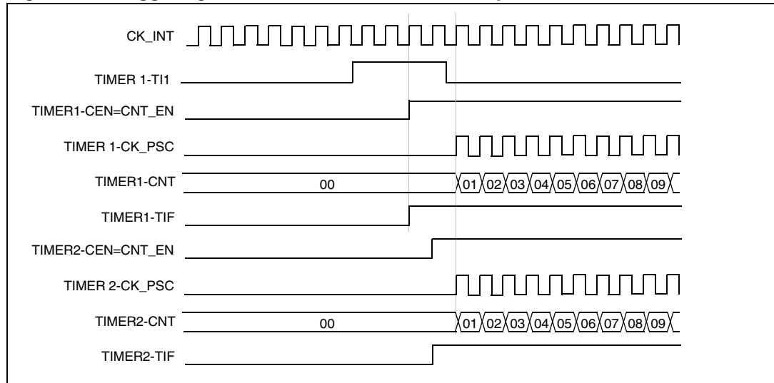
Figure 140. Triggering timer 1 and 2 with timer 1 TI1 input.
