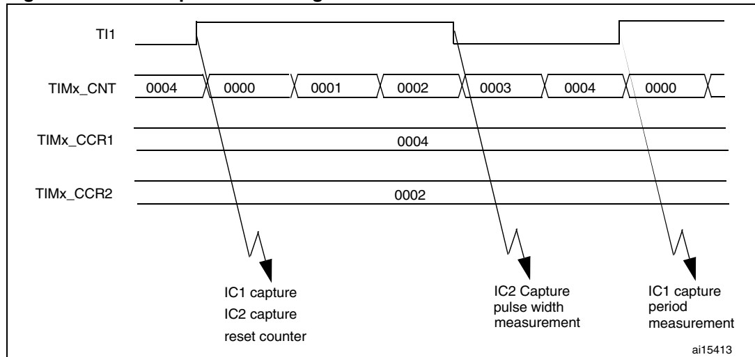
Figure 77. PWM input mode timing
