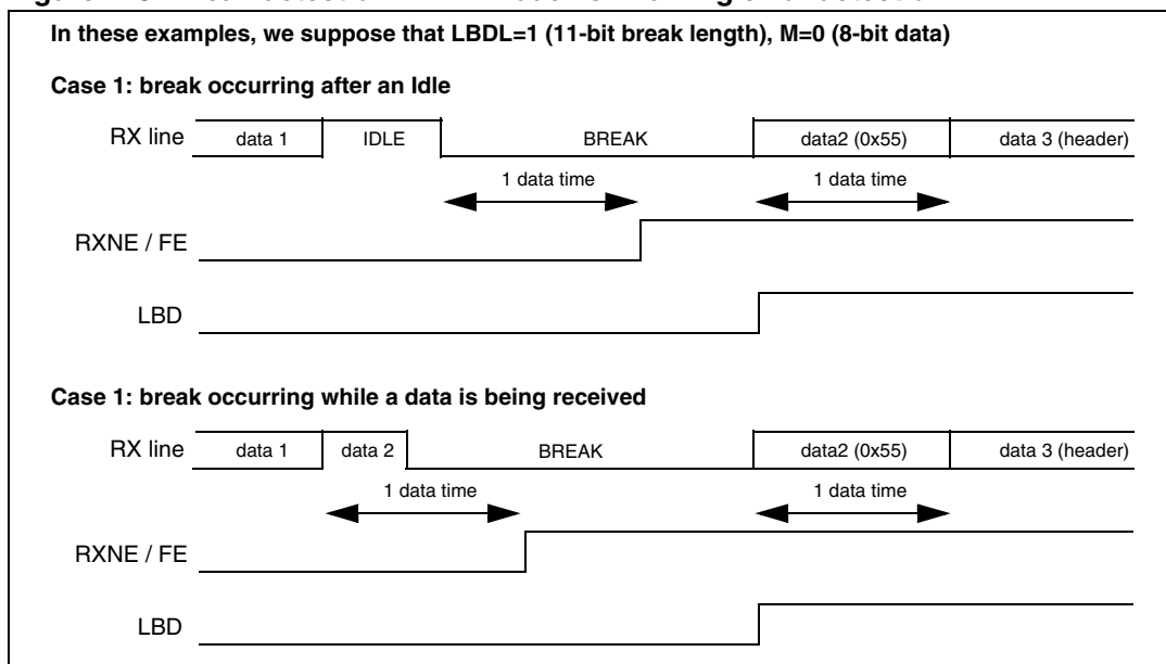
Figure 245. Break detection in LIN mode vs. Framing error detection
