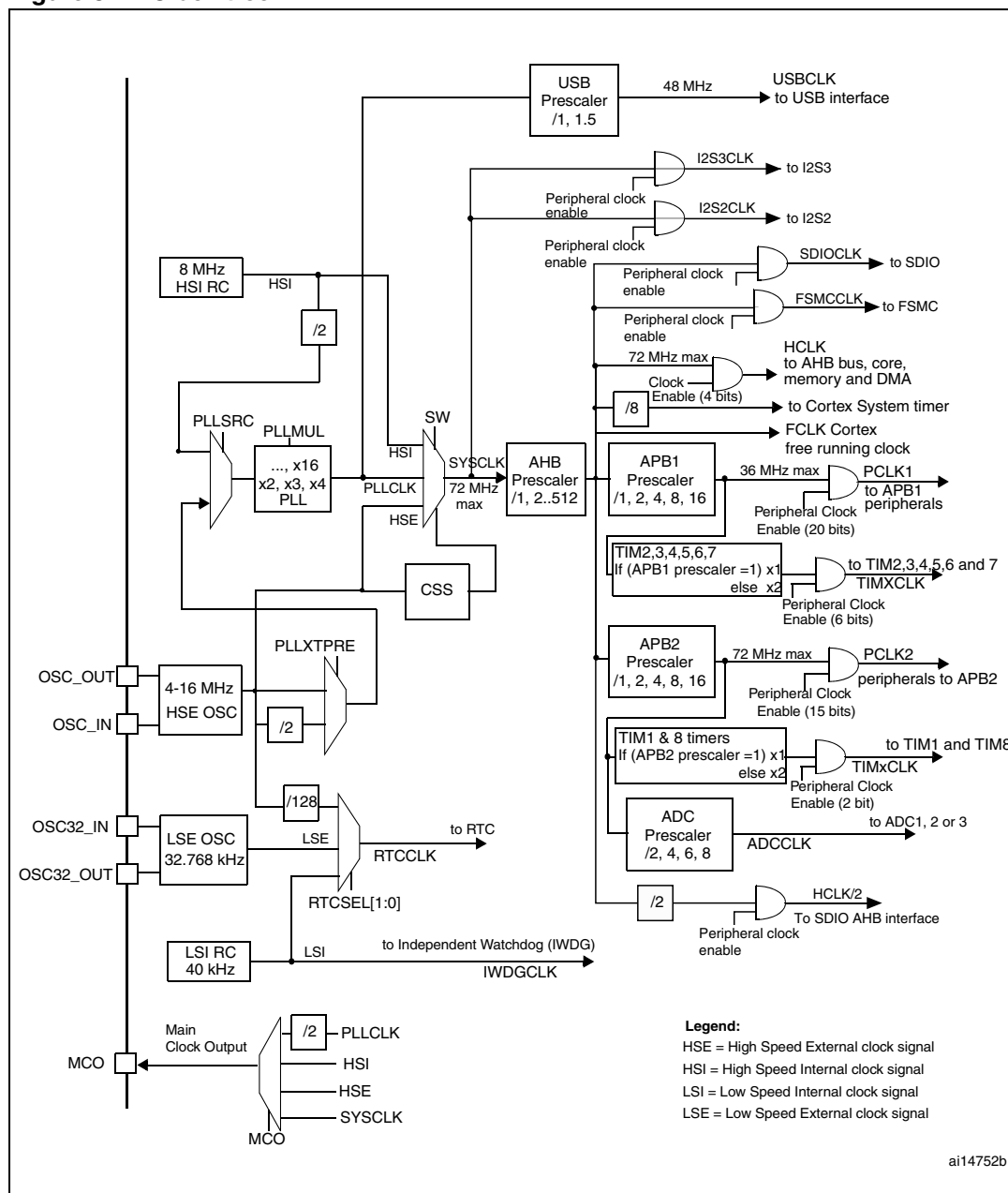
Figure 8. Clock tree
