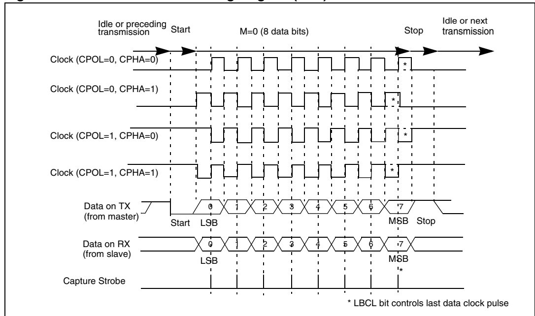
Figure 247. USART data clock timing diagram (M=0)
