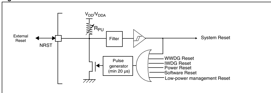
Figure 7. Reset circuit
