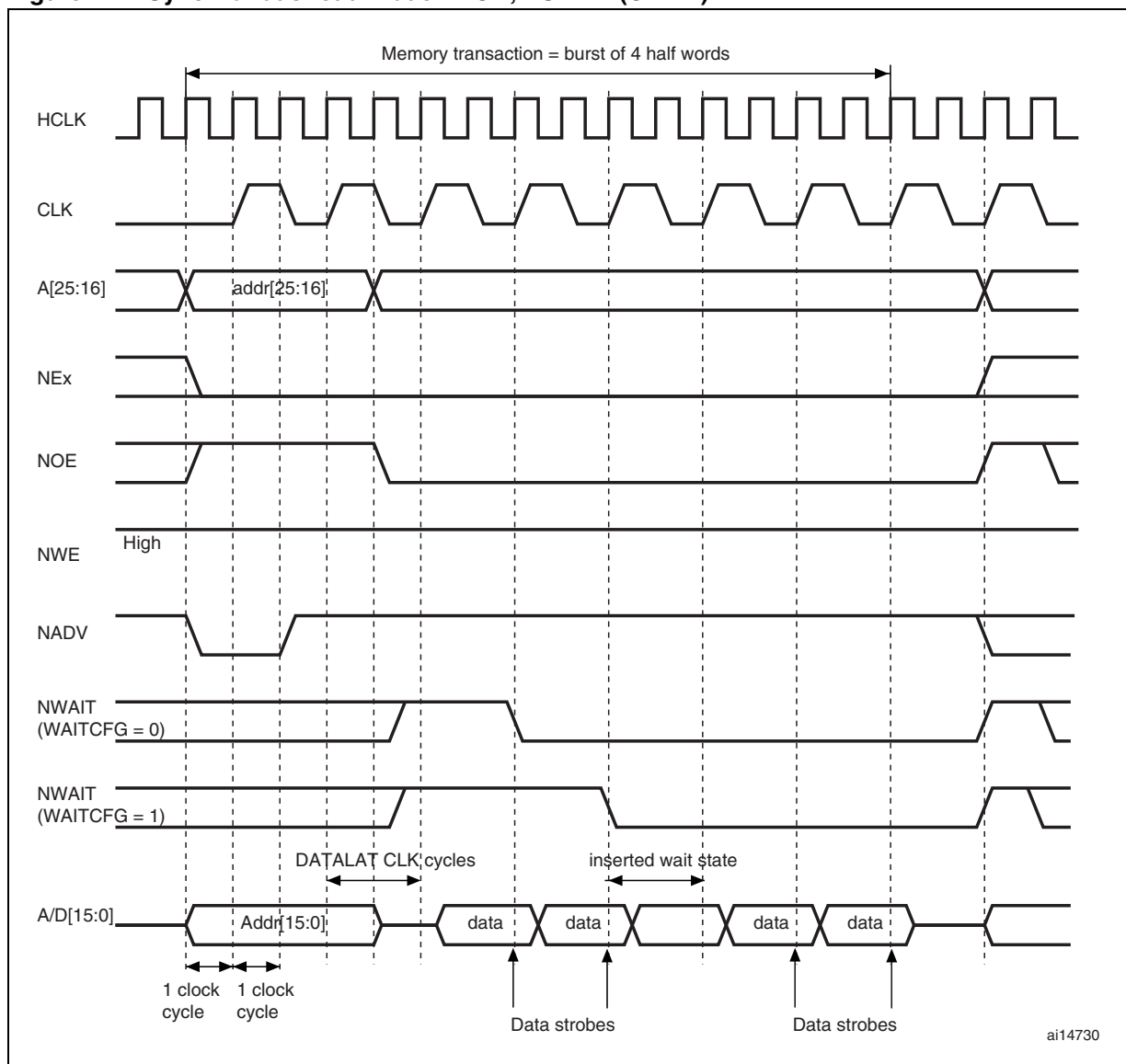
Figure 172. Synchronous read mode - NOR, PSRAM (CRAM)
