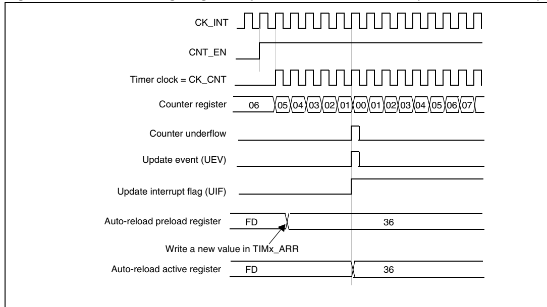
Figure 113. Counter timing diagram, Update event with ARPE=1 (counter underflow)
