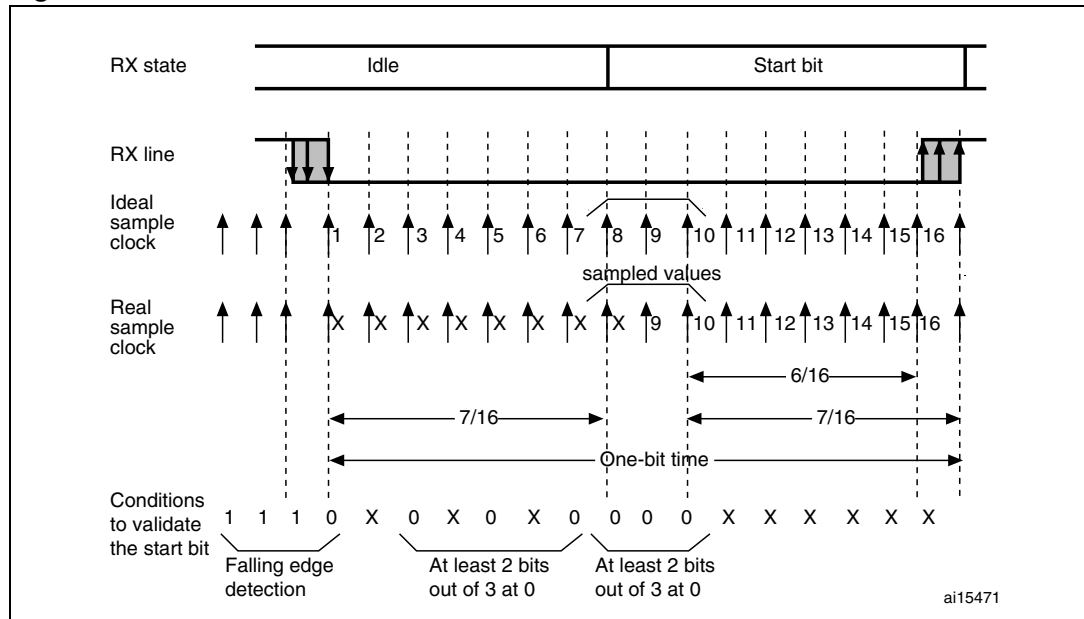
Figure 240. Start bit detection
