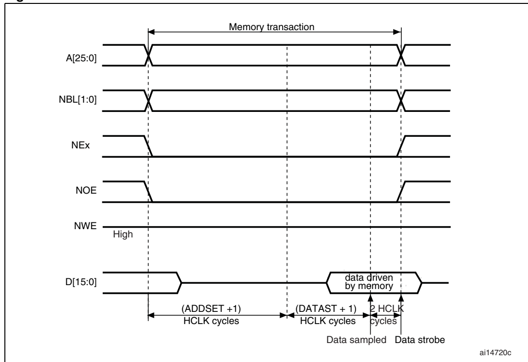
Figure 159. Mode1 read accesses
