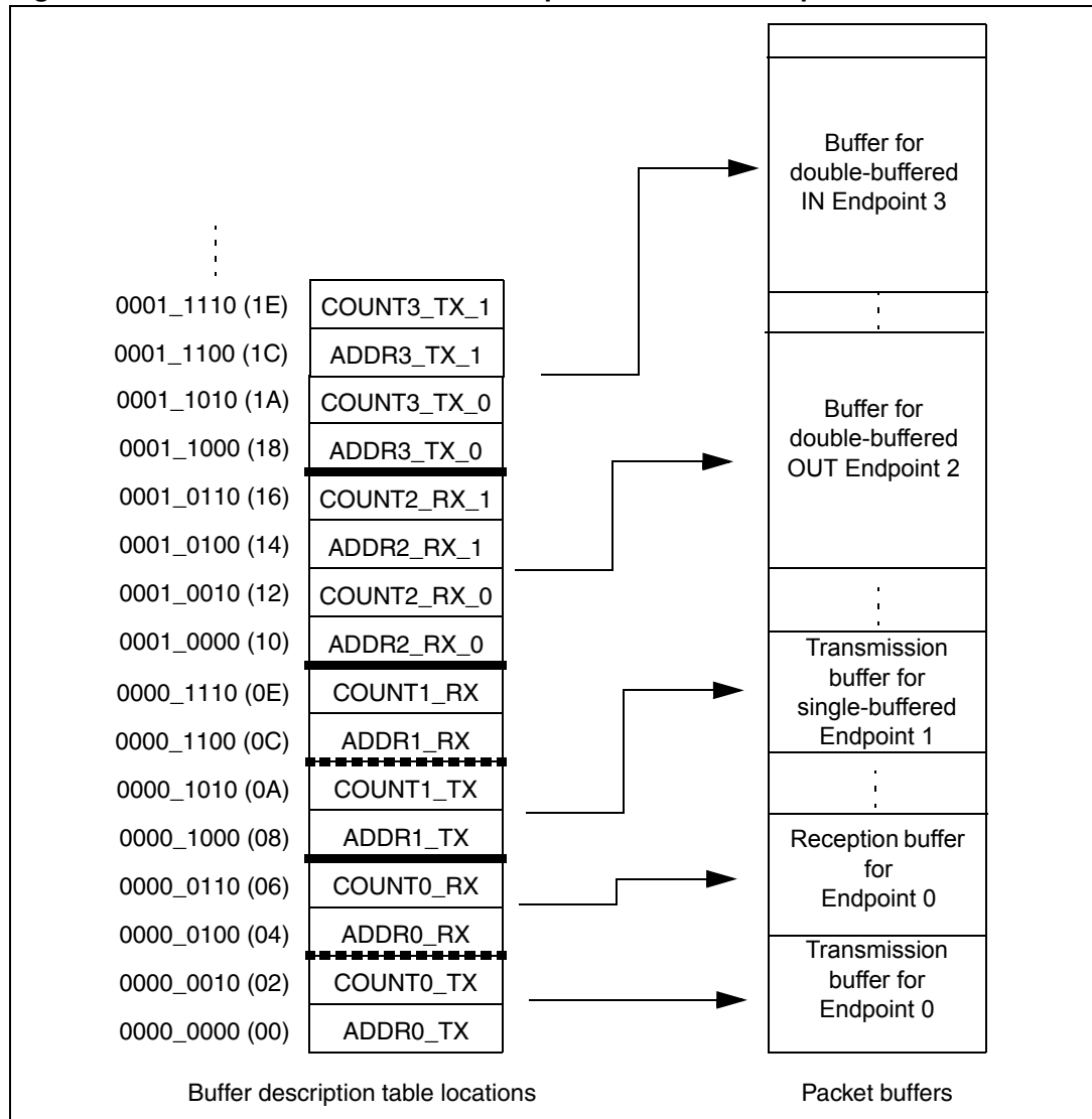
Figure 190. Packet buffer areas with examples of buffer description table locations
