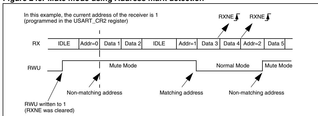
Figure 243. Mute mode using Address mark detection
