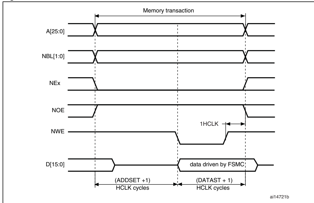
Figure 160. Mode1 write accesses
