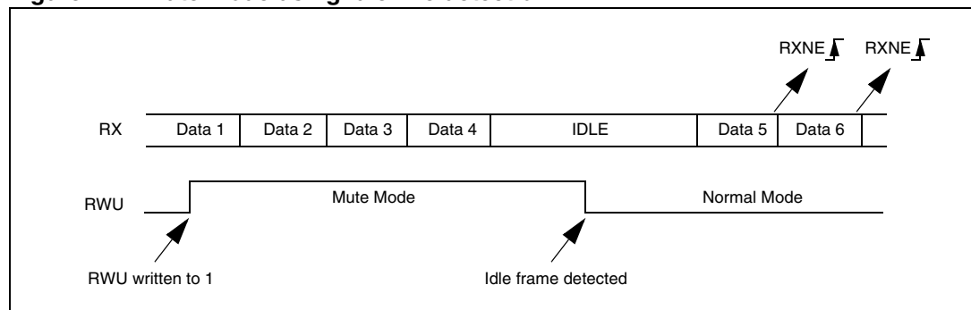
Figure 242. Mute mode using Idle line detection
