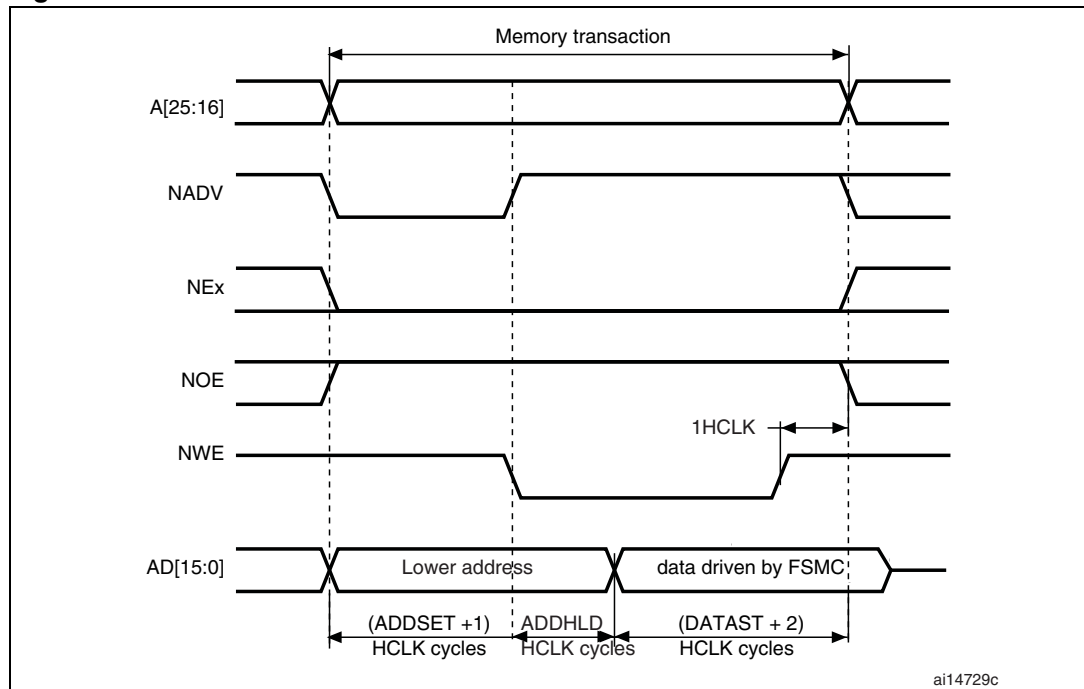
Figure 171. Muxed write accesses
