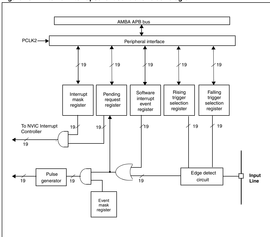
Figure 16. External interrupt/event controller block diagram
