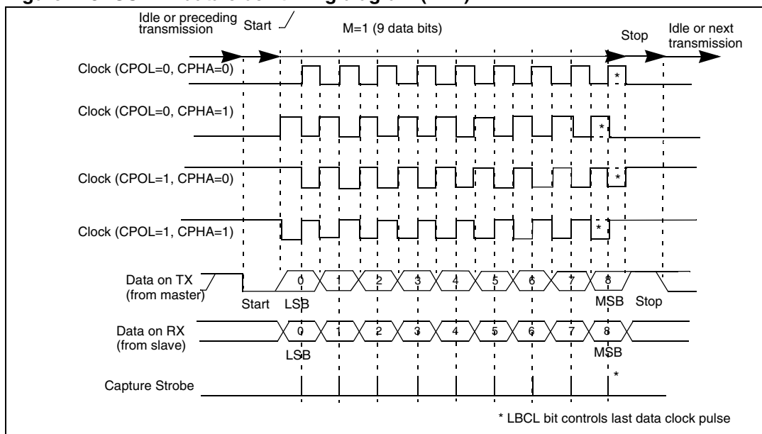
Figure 248. USART data clock timing diagram (M=1)
