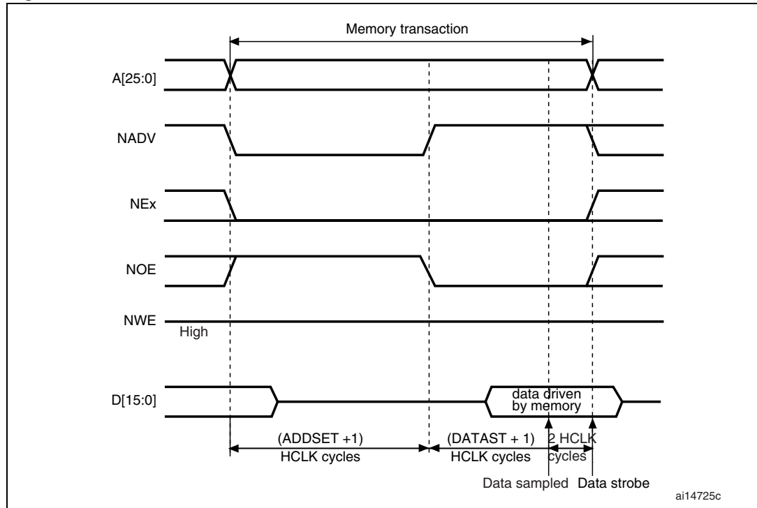
Figure 166. ModeC read accesses
