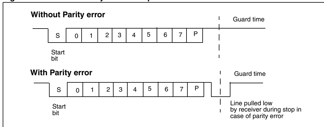
Figure 250. ISO 7816-3 asynchronous protocol
