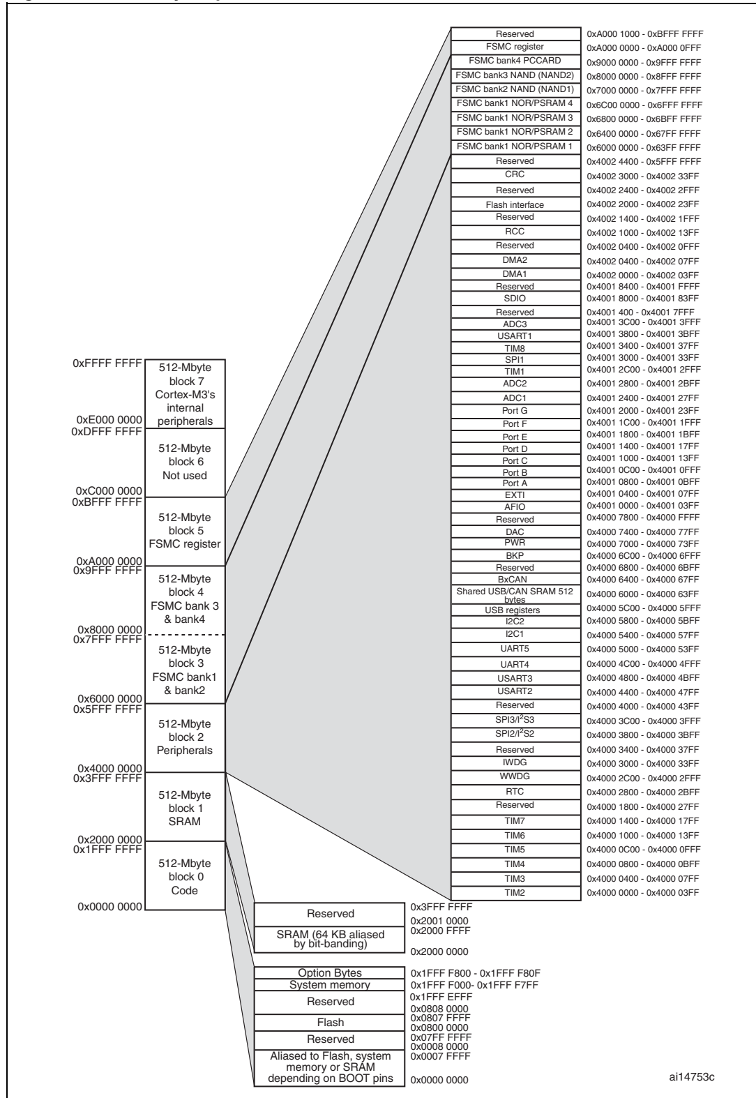
Figure 2. Memory map
