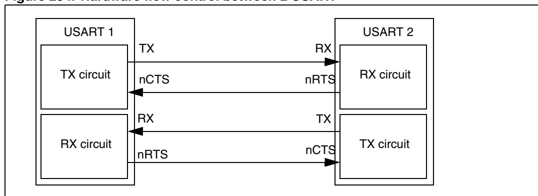
Figure 254. Hardware flow control between 2 USART
