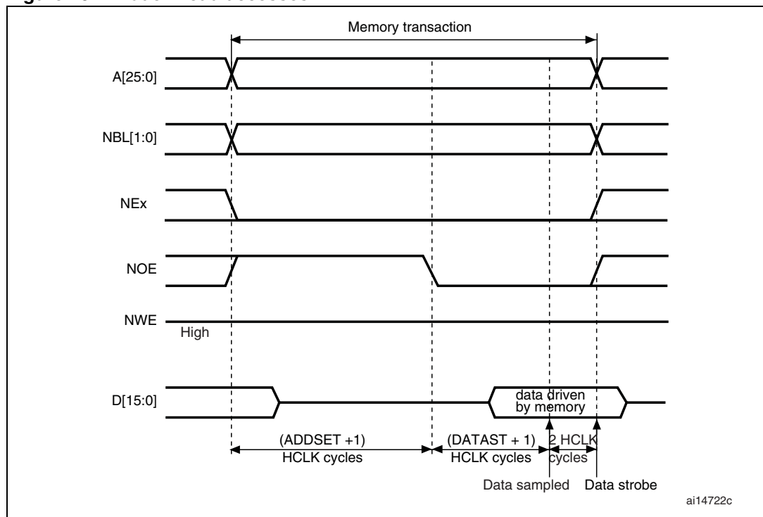
Figure 161. ModeA read accesses
