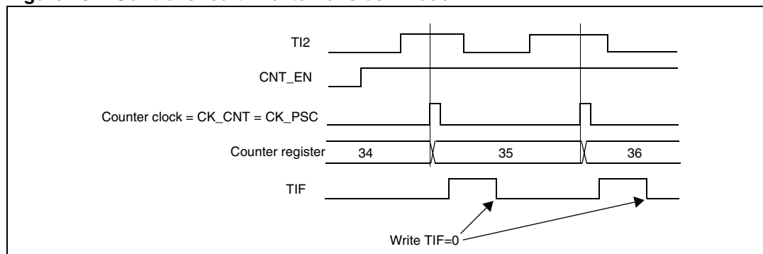
Figure 70. Control circuit in external clock mode 1
