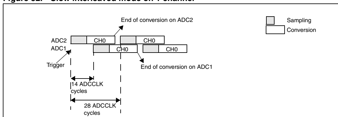
Figure 32. Slow interleaved mode on 1 channel
