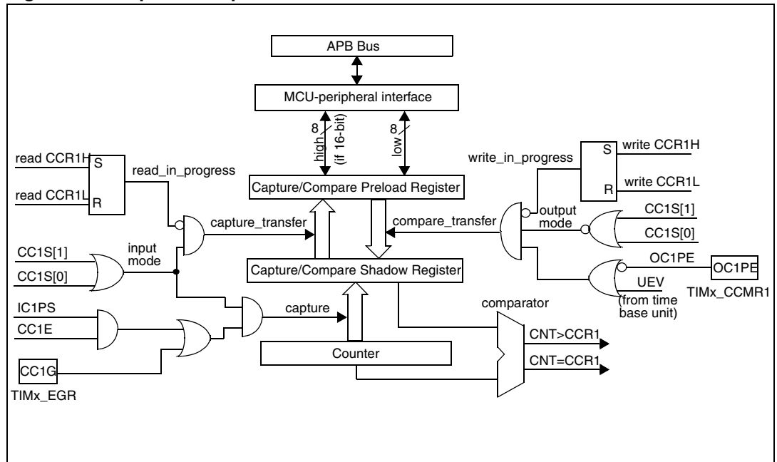
Figure 121. Capture/compare channel 1 main circuit
