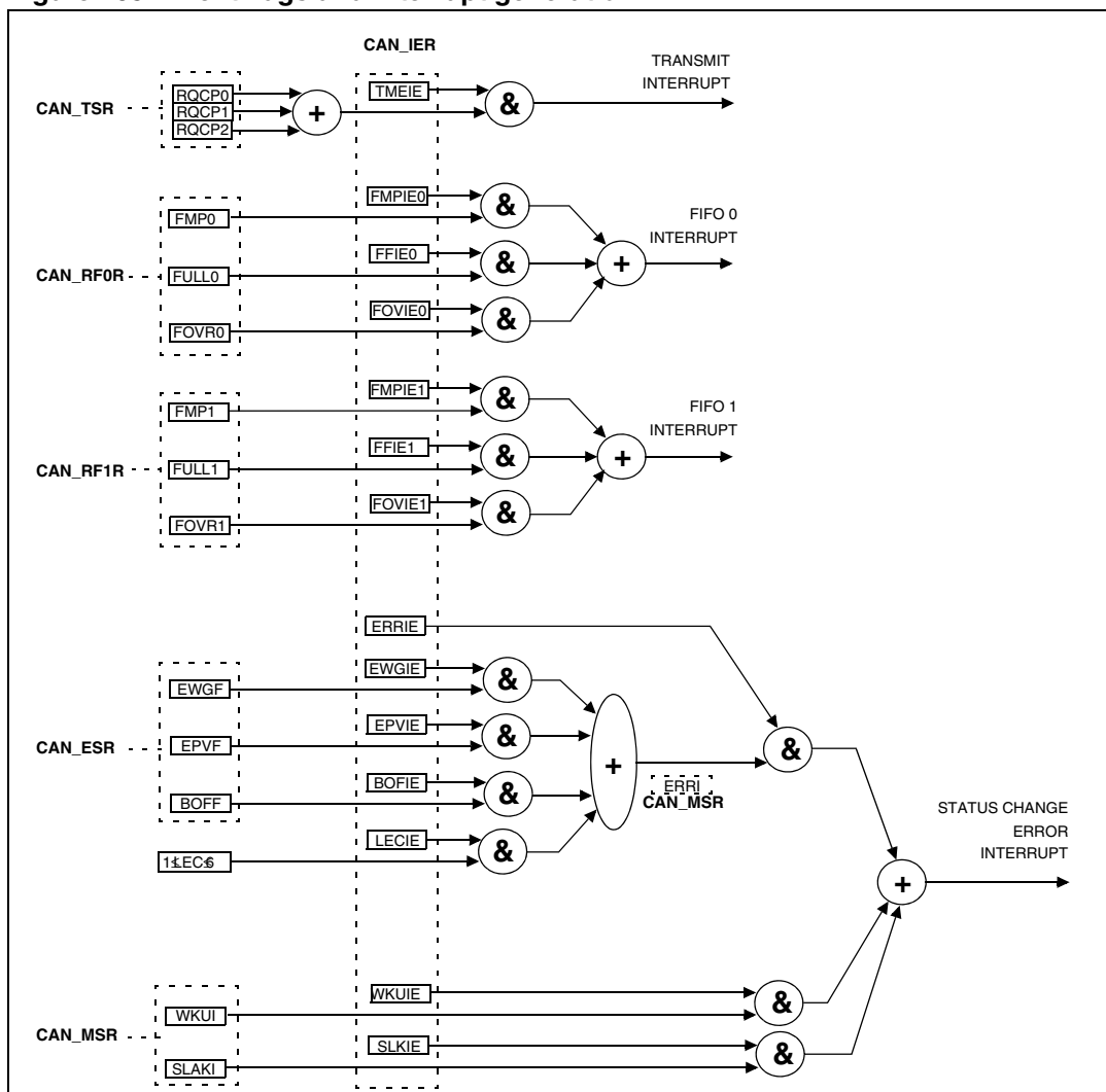
Figure 205. Event flags and interrupt generation
