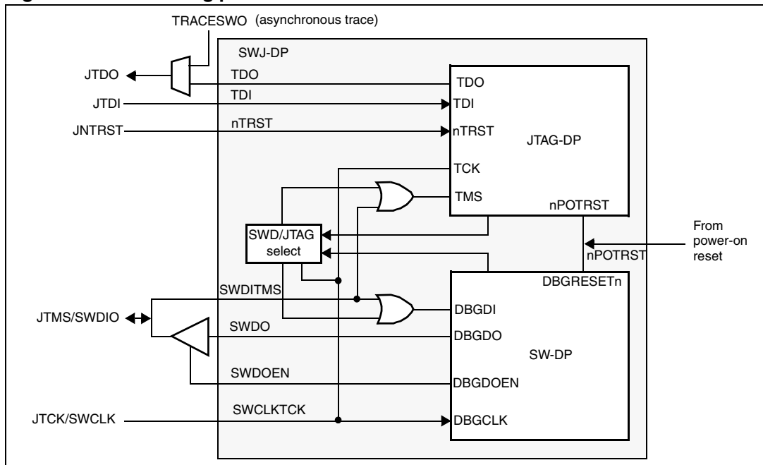
Figure 259. SWJ debug port
