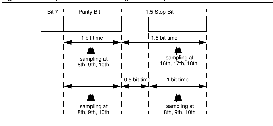
Figure 251. Parity error detection using the 1.5 stop bits
