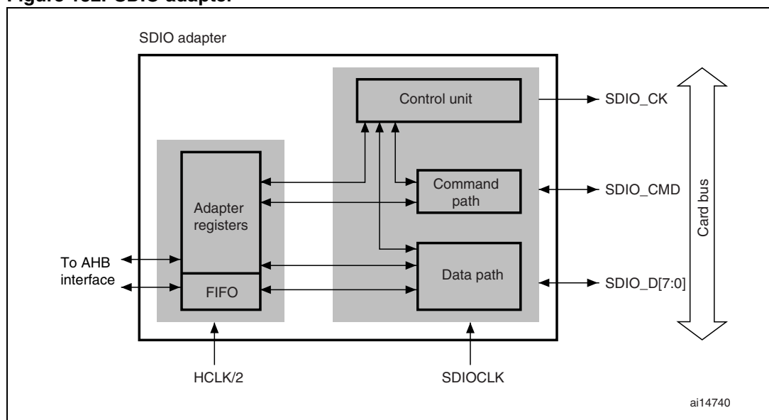
Figure 182. SDIO adapter
