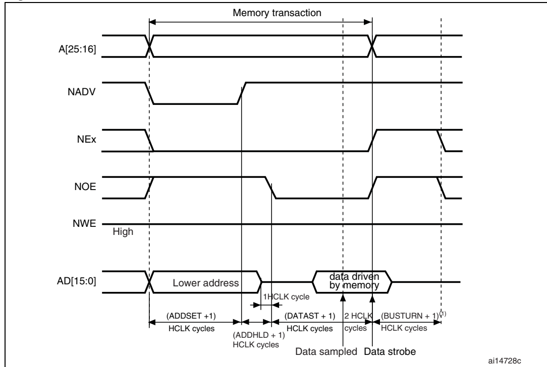
Figure 170. Muxed read accesses
