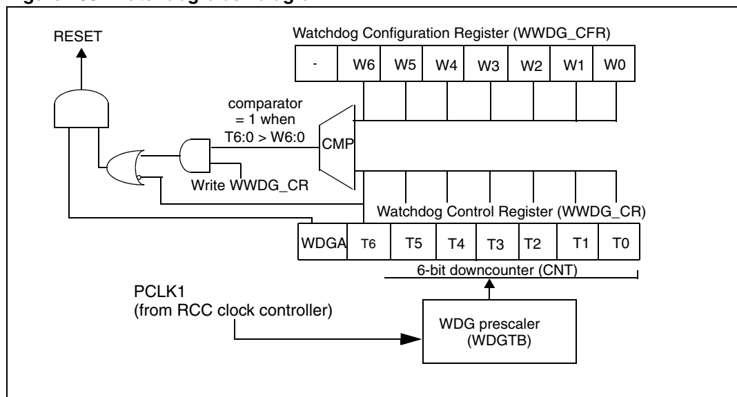
Figure 155. Watchdog block diagram
