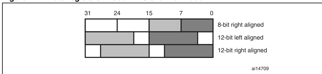
Figure 41. Data registers in dual DAC channel mode
