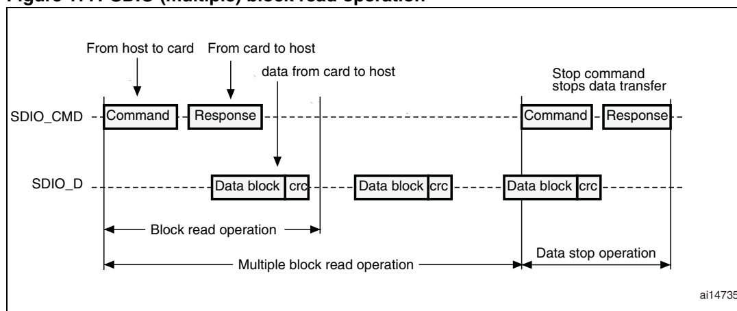
Figure 177. SDIO (multiple) block read operation
