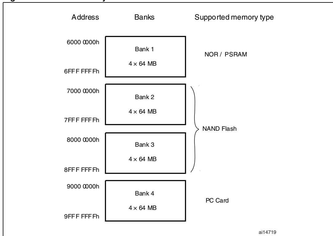
Figure 158. FSMC memory banks
