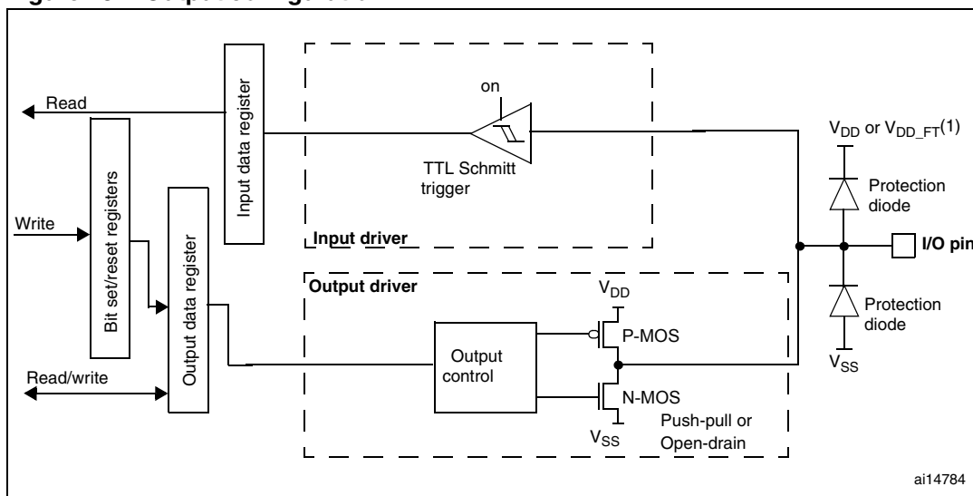
Figure 13. Output configuration
