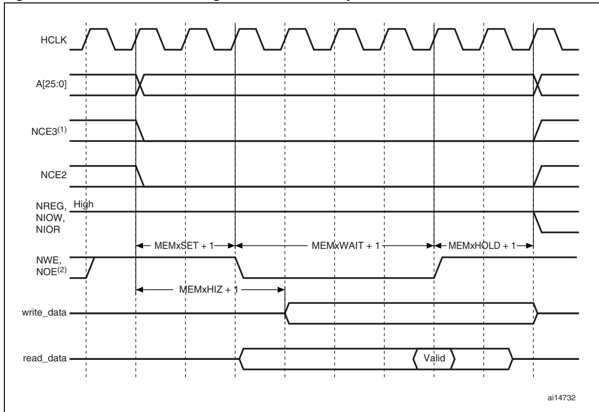
Figure 174. NAND controller timing for common memory access
