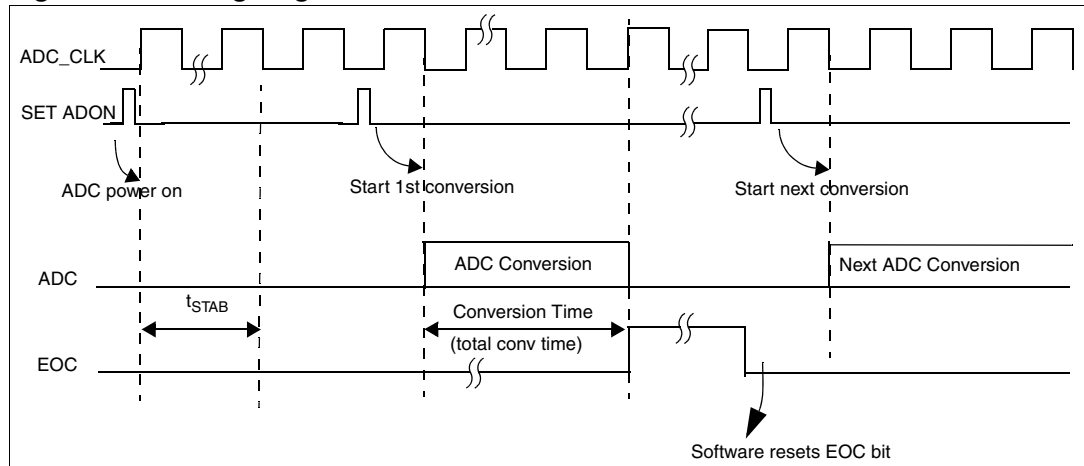
Figure 22. Timing diagram
