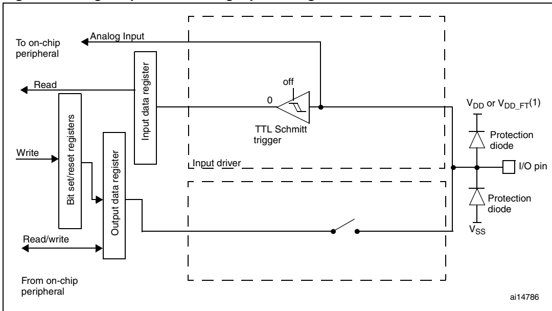
Figure 15. High impedance-analog input configuration
