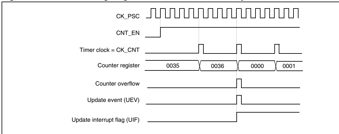
Figure 53. Counter timing diagram, internal clock divided by N
