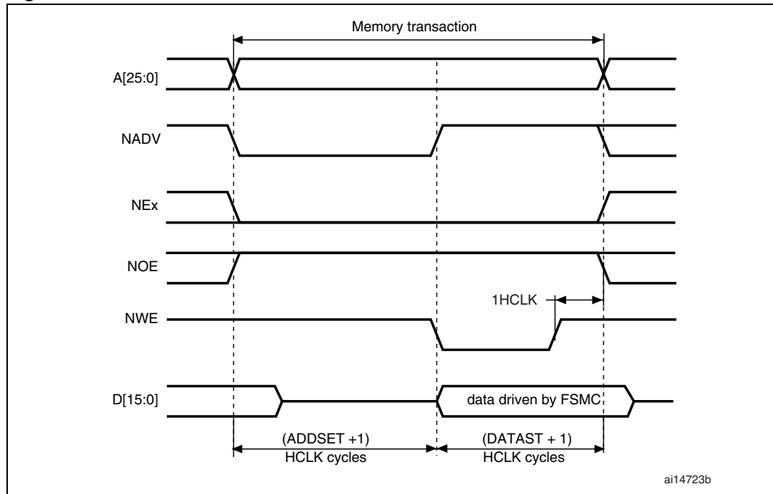
Figure 164. Mode2 write accesses
