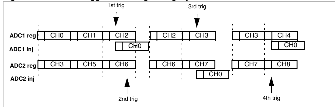
Figure 36. Case of trigger occurring during injected conversion
