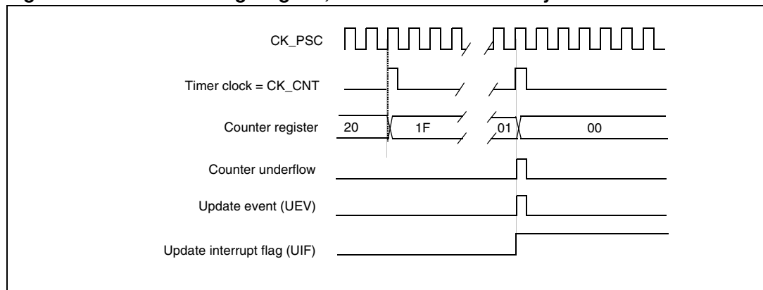
Figure 65. Counter timing diagram, update event with ARPE=1 (counter underflow)
