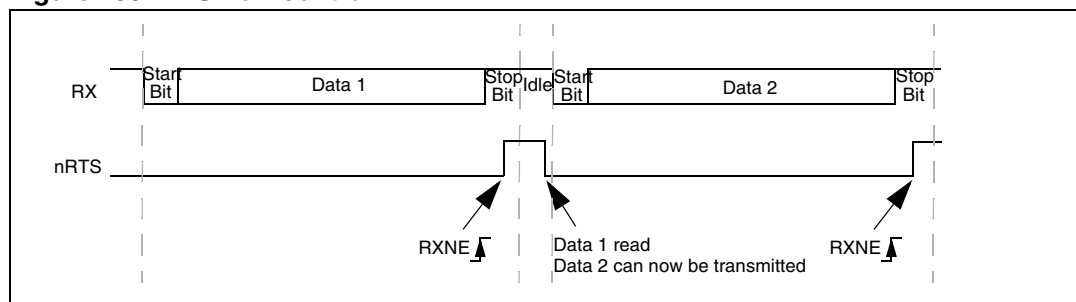
Figure 255. RTS flow control
