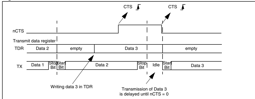
Figure 256. CTS flow control
