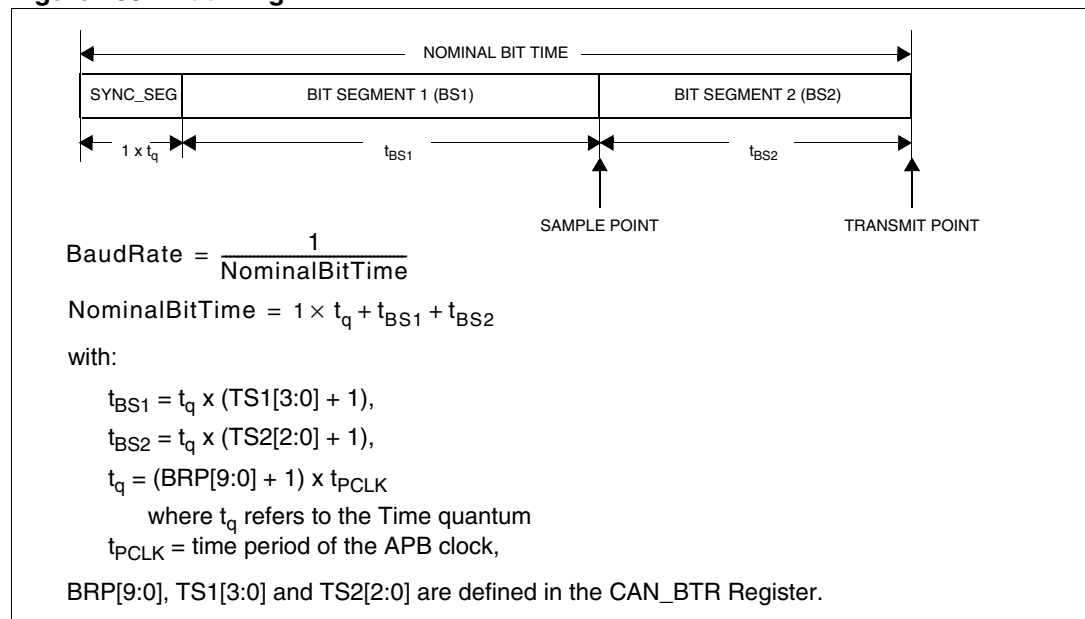
Figure 203. Bit timing
