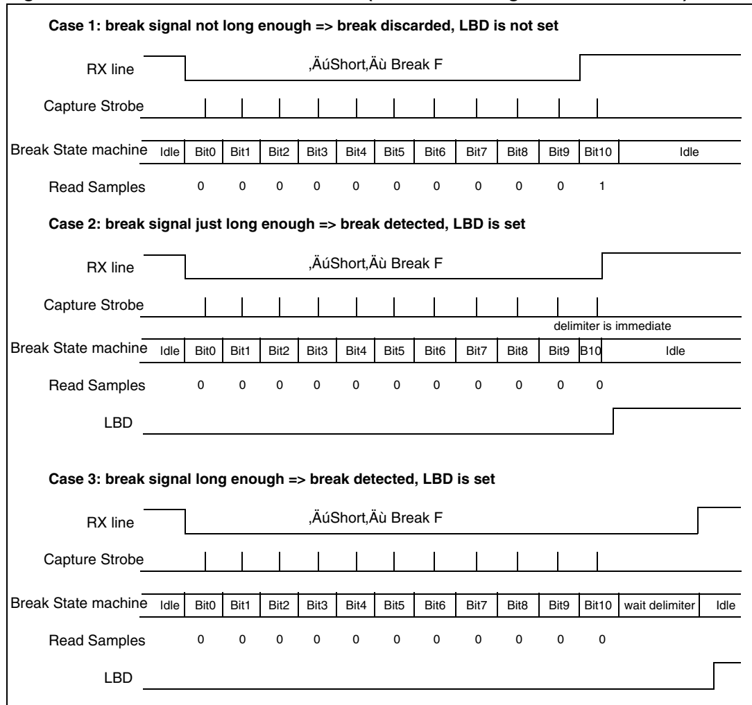
Figure 244. Break detection in LIN mode (11-bit break length - LBDL bit is set)
