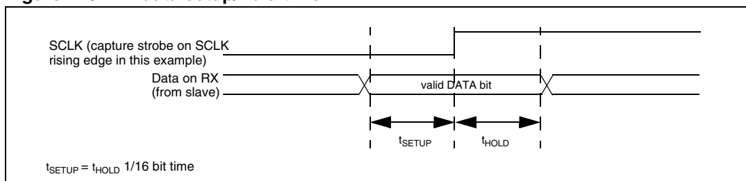
Figure 249. RX data setup/hold time
