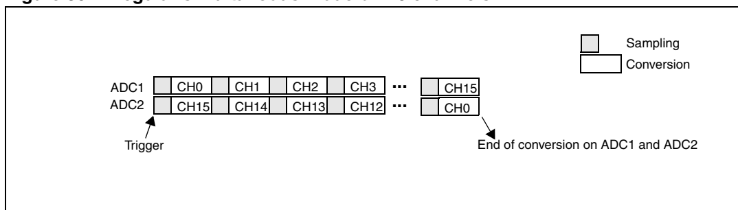
Figure 30. Regular simultaneous mode on 16 channels
