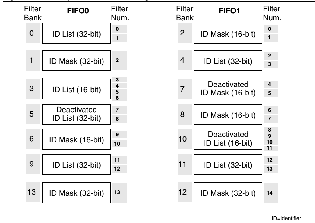
Figure 200. Example of filter numbering
